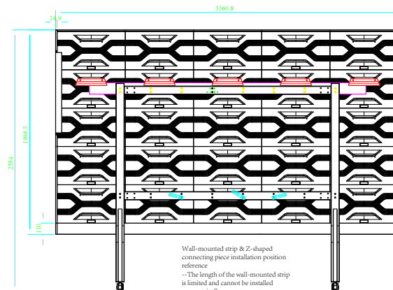
Installation diagram on the back of the screen
