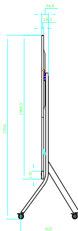
Screen side installation diagram
