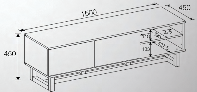
Dimensions (mm)
