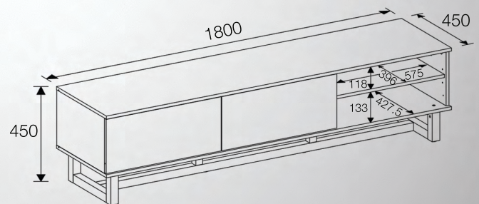
Dimensions (mm)
