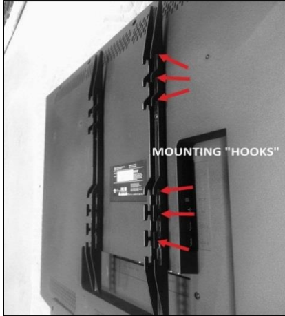
Vertical Mounting Bars attached to back of TV
