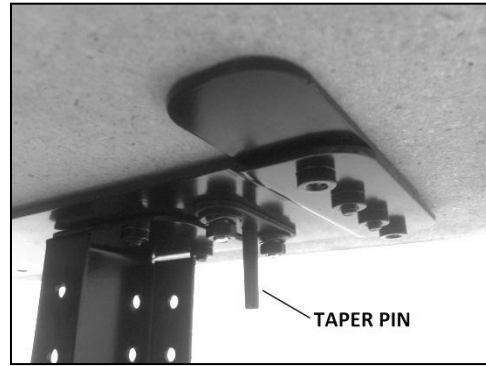
Tapered Pin passing through Top Plate
