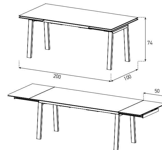
TANDEM MOVE UP
