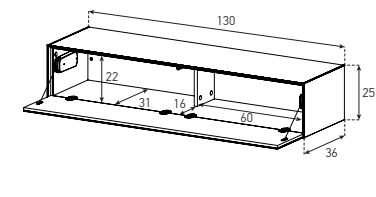
ED66F (WITH CABLE MANAGEMENT)
