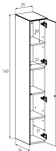
ED95DR / DL (Adjustable shelf +/- 6 cm)
