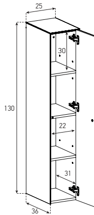
ED81DR / DL (Removable shelf)
