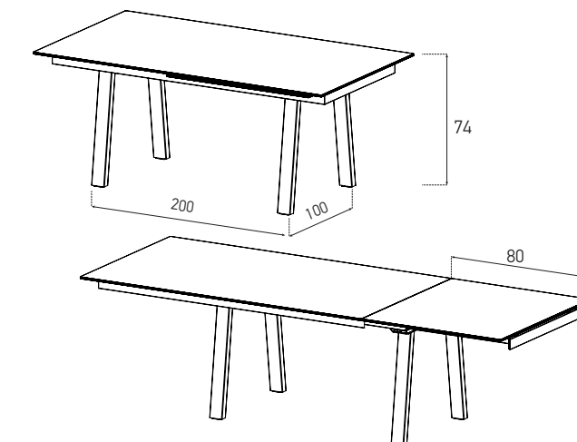
TANDEM MOVE UP
