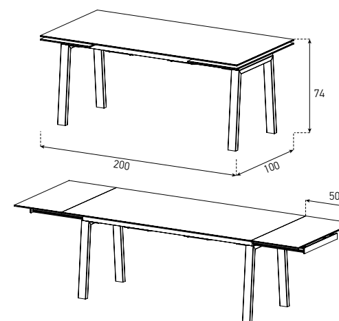
LIFT OPENING(ALU)
