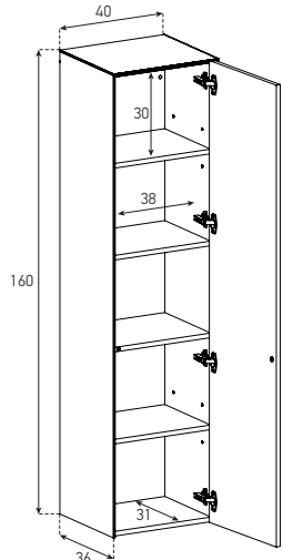
ED95DR / DL (Adjustable shelf +/- 6 cm)
