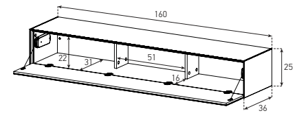
ED36F (WITH CABLE MANAGEMENT)
