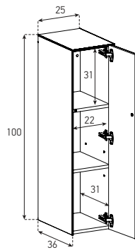
ED71DR / DL (Removable shelf)
