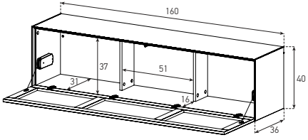
ED31TS / PS(WITH CABLE MANAGEMENT)
