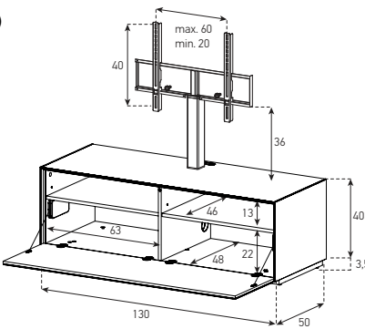
EX11F (Adjustable shelf + 4 cm)
