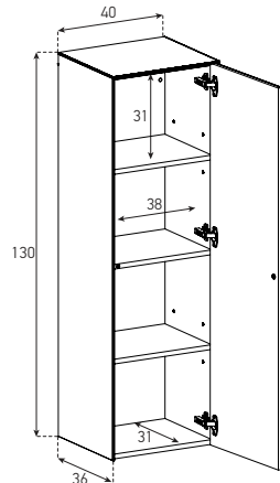
ED85DR / DL (Adjustable shelf +/- 6 cm)
